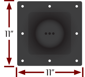
BASE (BOTTOM)
