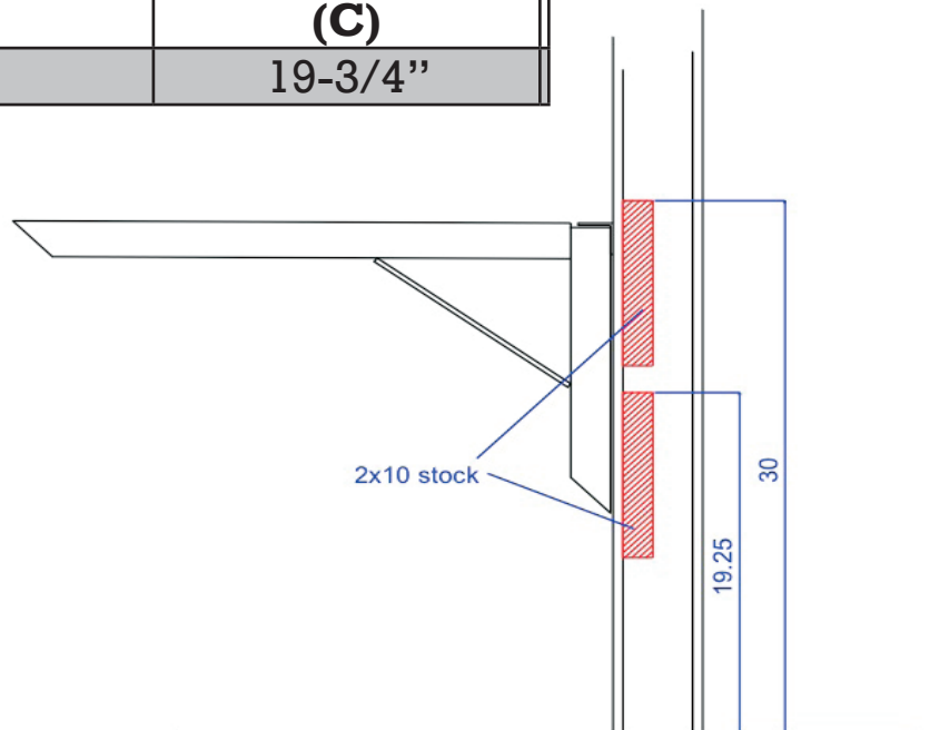
Wall backing for cantilever bases
